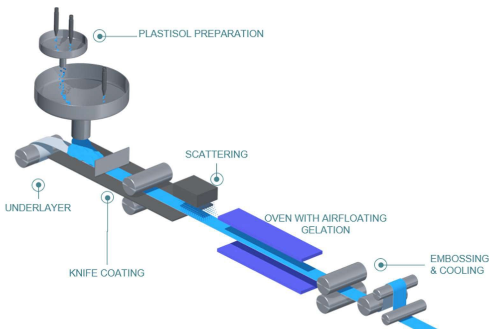
Figure 3: Coating process
